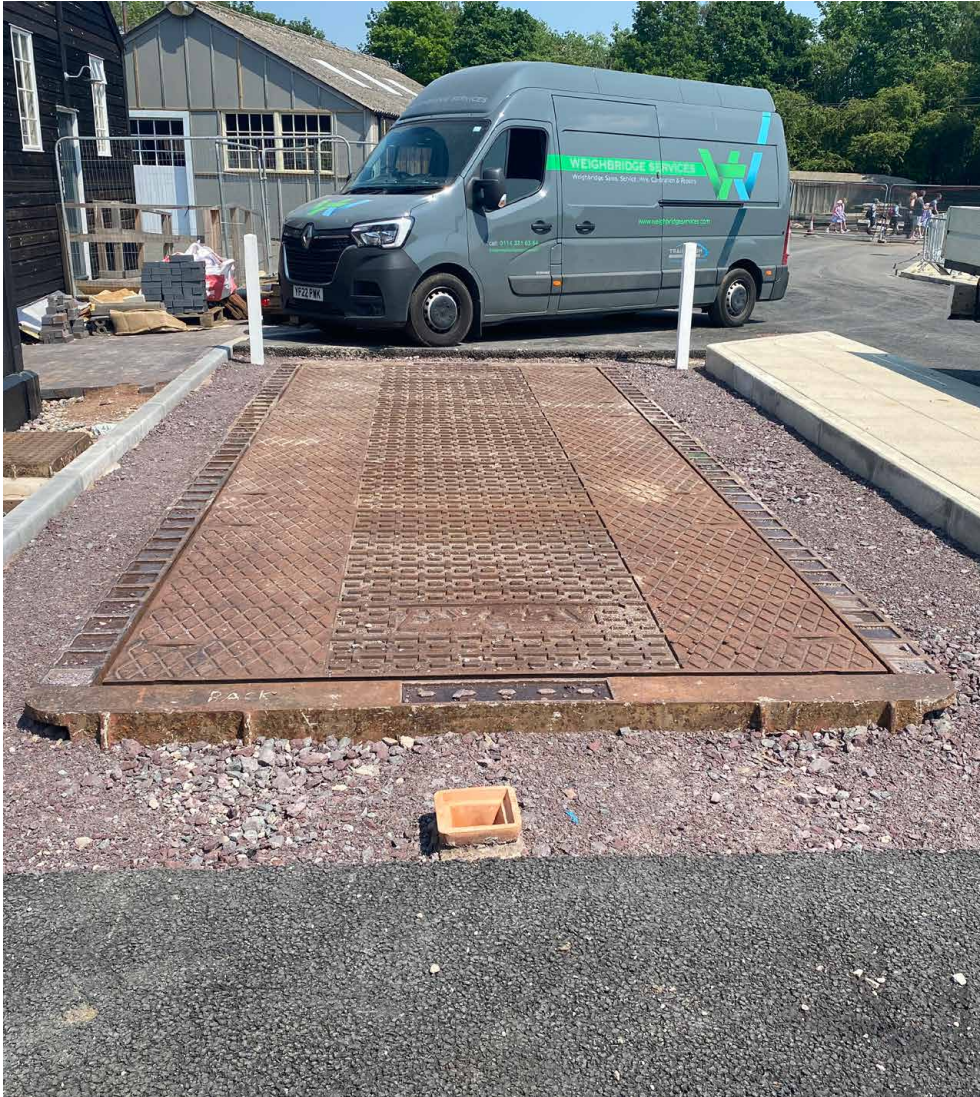
Project: Conversion of an old mechanical weighbridge installed at Black Country Living Museum, Dudley
