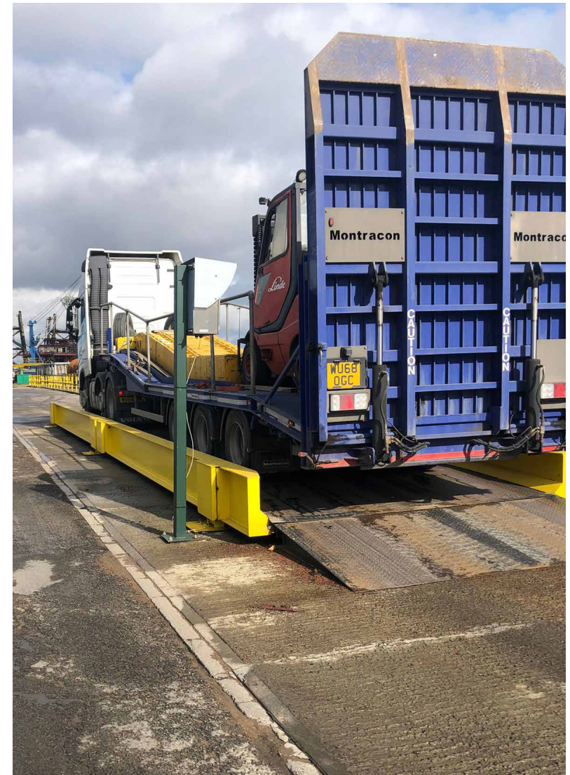
Project: Calibration test unit at Port of Blyth, Battleship Wharf
